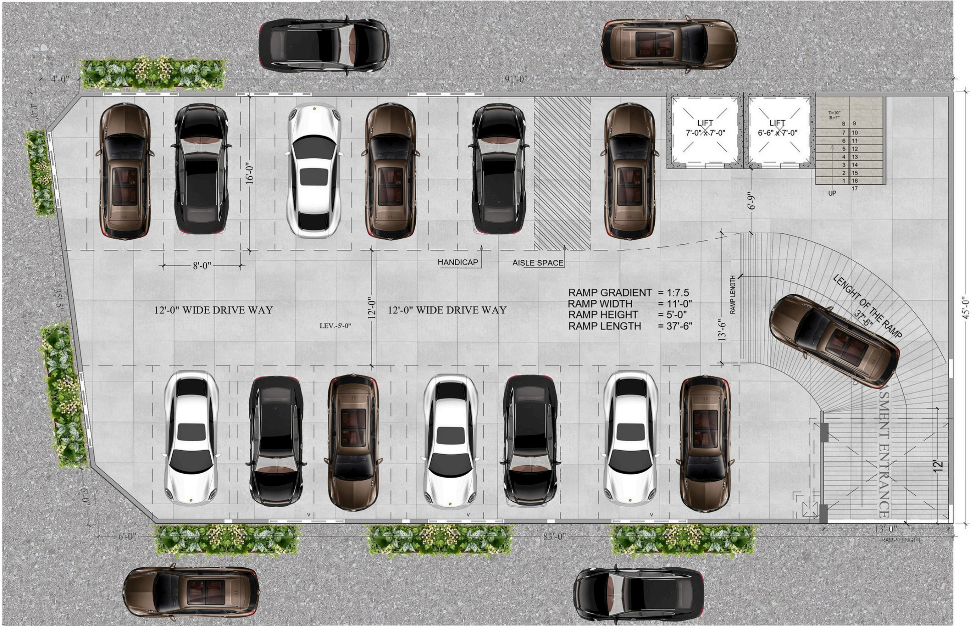
BASEMENT PLAN
